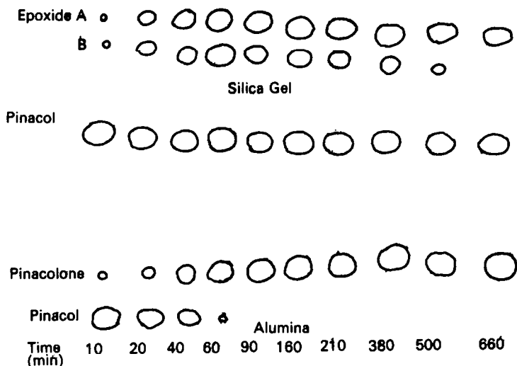
FIG. 1 The thin layer chromatogram of the reaction products of meso -2,2'-dimethylbenzpinacol (0.00942 mole) in 2.64 \times 10^{-4} mole- \text{HClO}_4 -acetic acid at 72^\circ . Developer: Benzene + Hexane (1:2)
