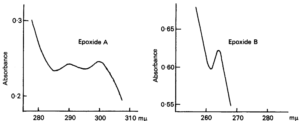
FIG. 4 UV spectra of cis - and trans -1,2-diphenyl-1,2-ditolyl-ethylene oxide in ethanol.
