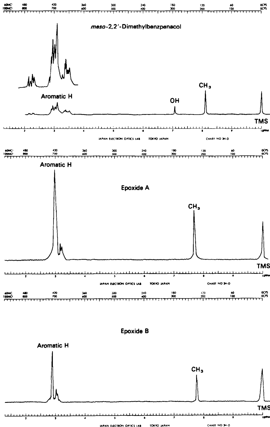
FIG. 3 PMR spectra of cis - and trans -1,2-diphenyl-1,2-ditolylethylene oxide in carbon tetrachloride.
