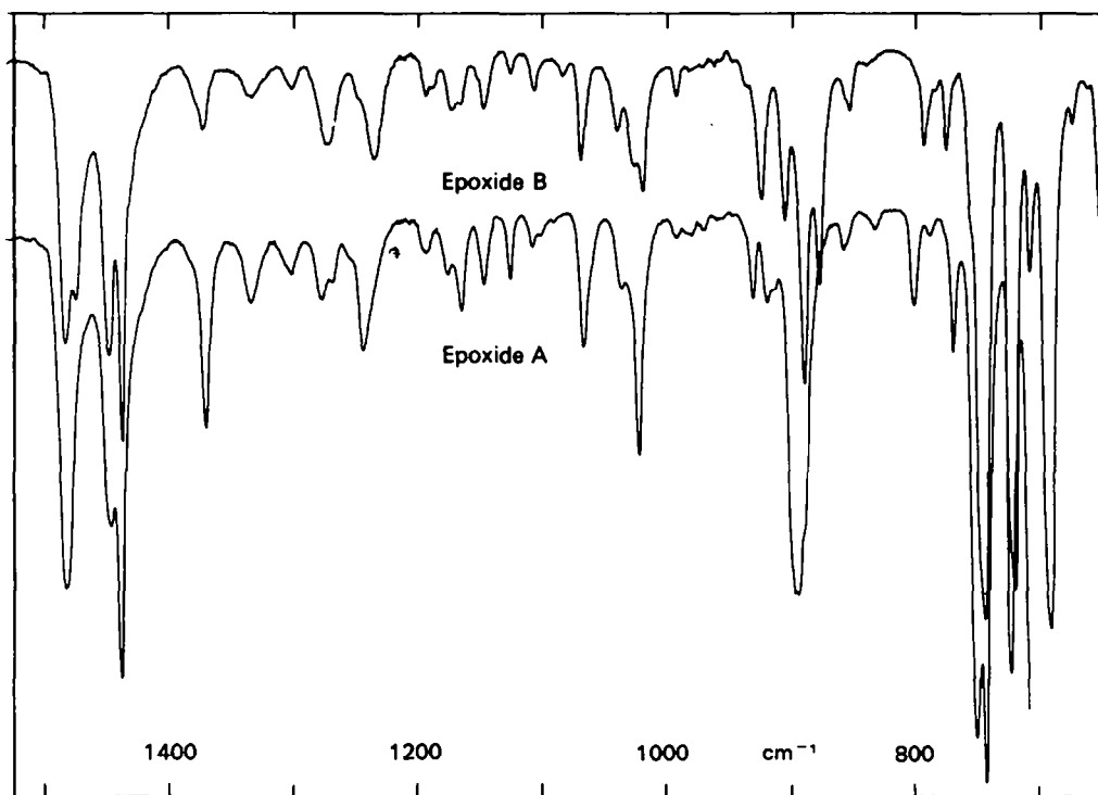
FIG. 2 IR spectra of cis - and trans -1,2-diphenyl-1,2-ditolylethylene oxides
