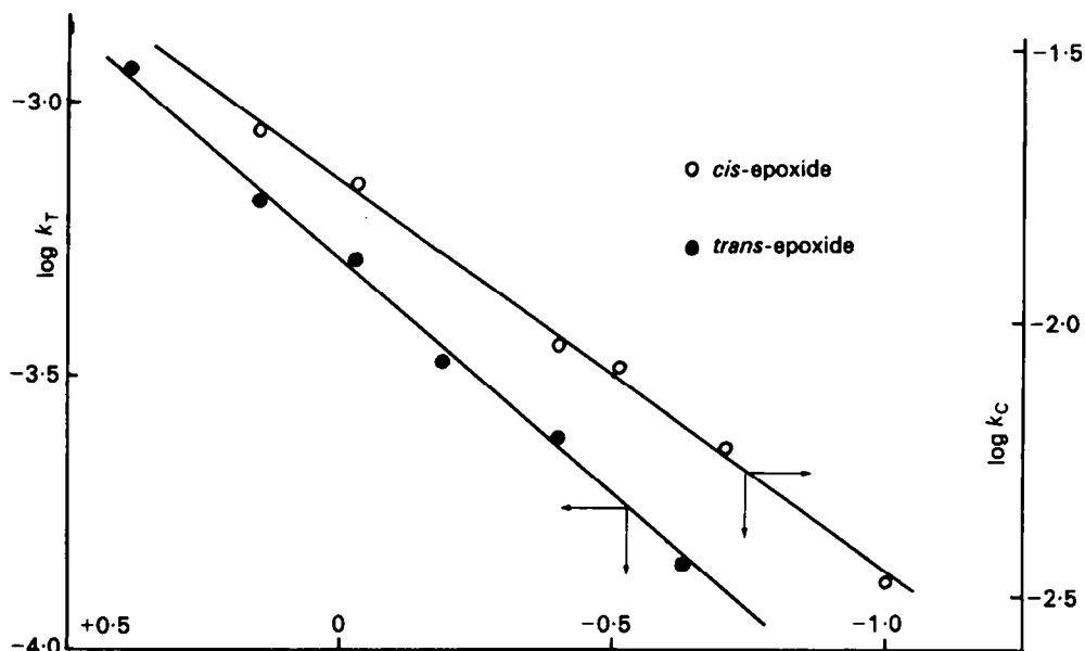
FIG. 6 Correlation of first order rate constant with the Hammett acidity function of the medium at 72°
