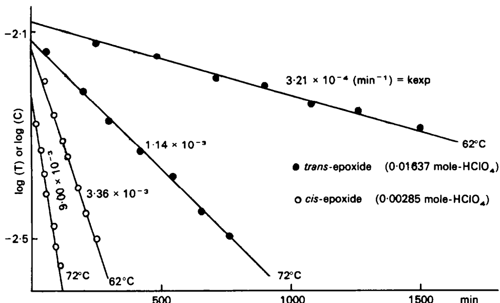
FIG. 5 The slopes of the straight lines obtained by plotting \log (C) or \log (T) vs. time (min) in the reaction of cis - and trans -1,2-diphenyl-1,2-ditolylethylene oxide.
